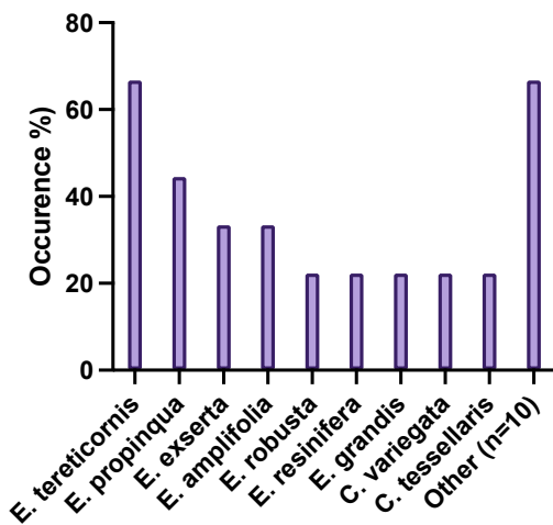
Frequency of detection in scats
