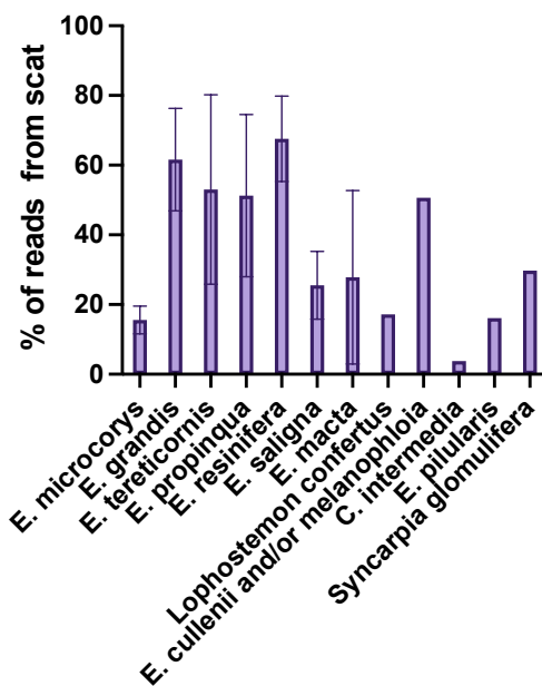
Mean contribution to scat
